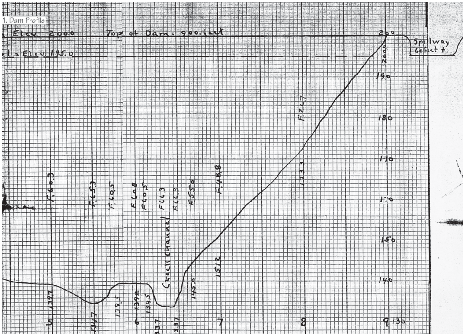
Figure 1b. Dam Profile, south
