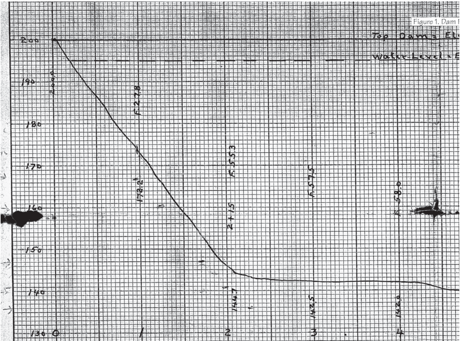
Figure 1a. Dam Profile, north
